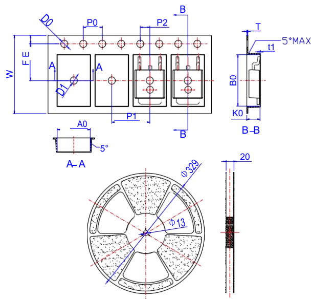
Reel Specification-TO-252
